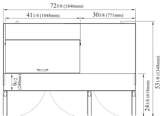
TST-72SD-18M-N TOP VIEW
