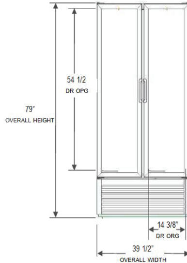
ELEVATION VIEW
