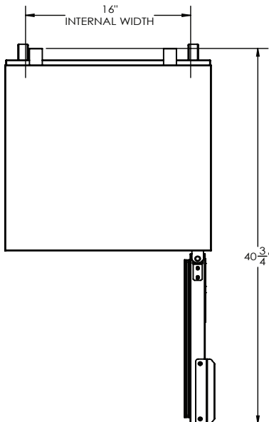
PLAN VIEW
