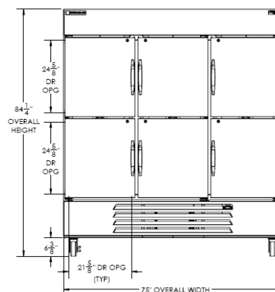
Elevation View
