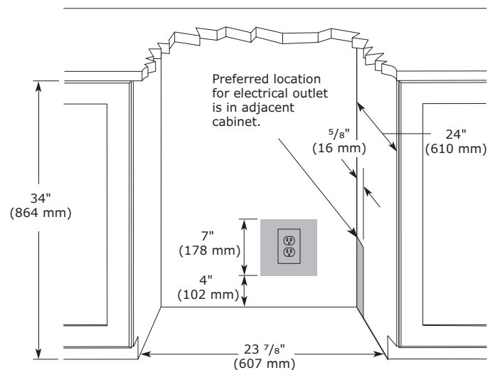
Cabinet Cut-Out
