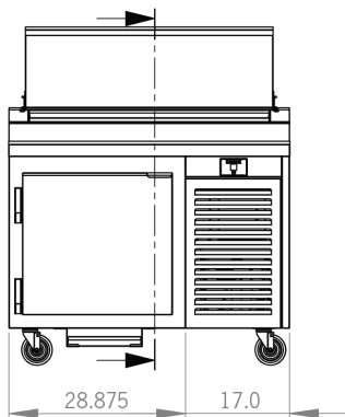
ELEVATION VIEW
