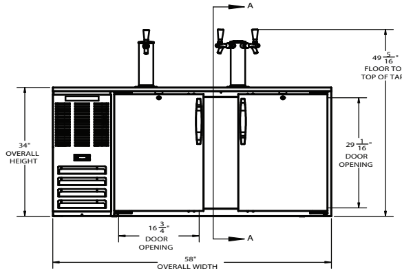
ELEVATION VIEW
