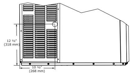
Back Panel
