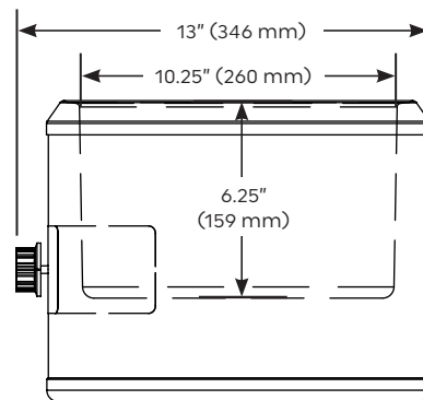
11Qt - SIDE VIEW
