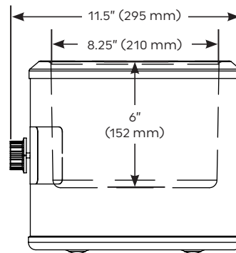
7Qt - SIDE VIEW
