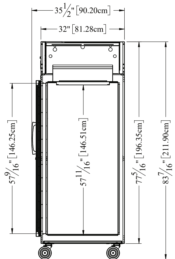
SIDE VIEW
