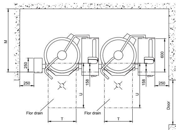
A. Water and steam connections from rear
