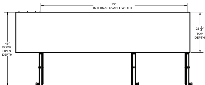
ELEVATION VIEW
