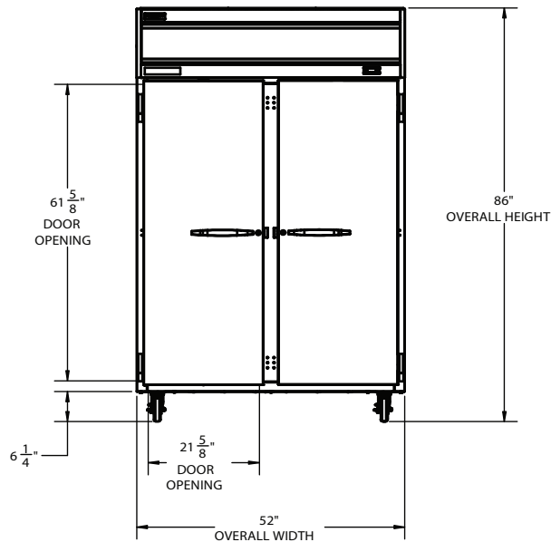
ELEVATION VIEW
