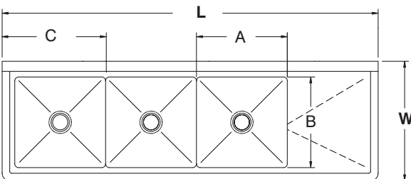
3 COMP - 1 DRBD
