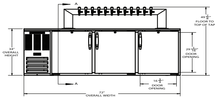
ELEVATION VIEW
