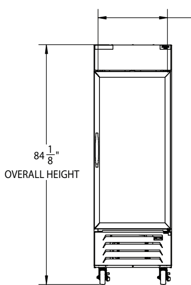
ELEVATION VIEW
