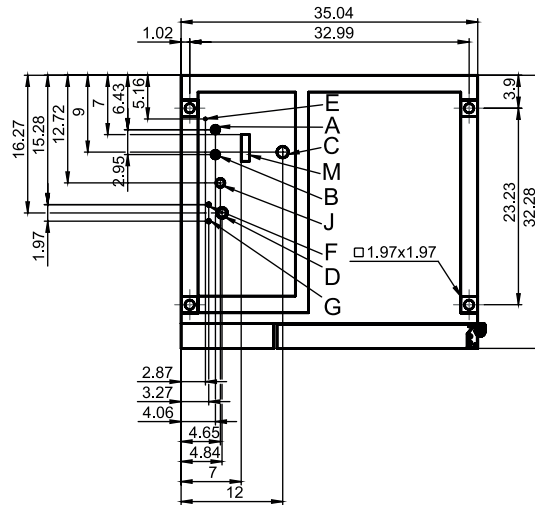
Connection points, bottom of unit
