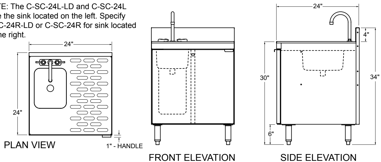
C-SC-24L OR R-LD (LESS DOOR), C-SC-24L OR R (LEFT SHOWN)
