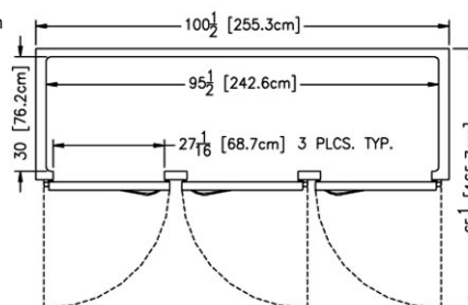
Plan - R/ARI334LUT
