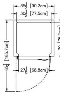
Plan - R/ARI134LUT
