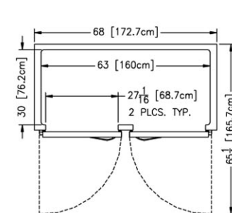
Plan - R/ARI234LUT
