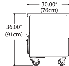
Right Side View All Models *Shown with optional cord hook
