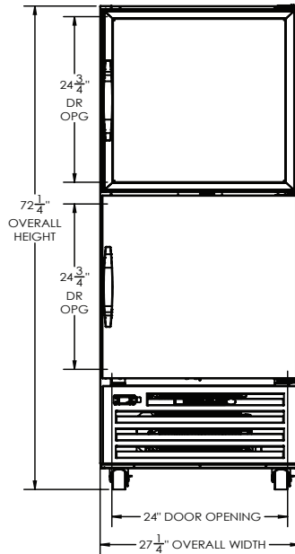
ELEVATION VIEW
