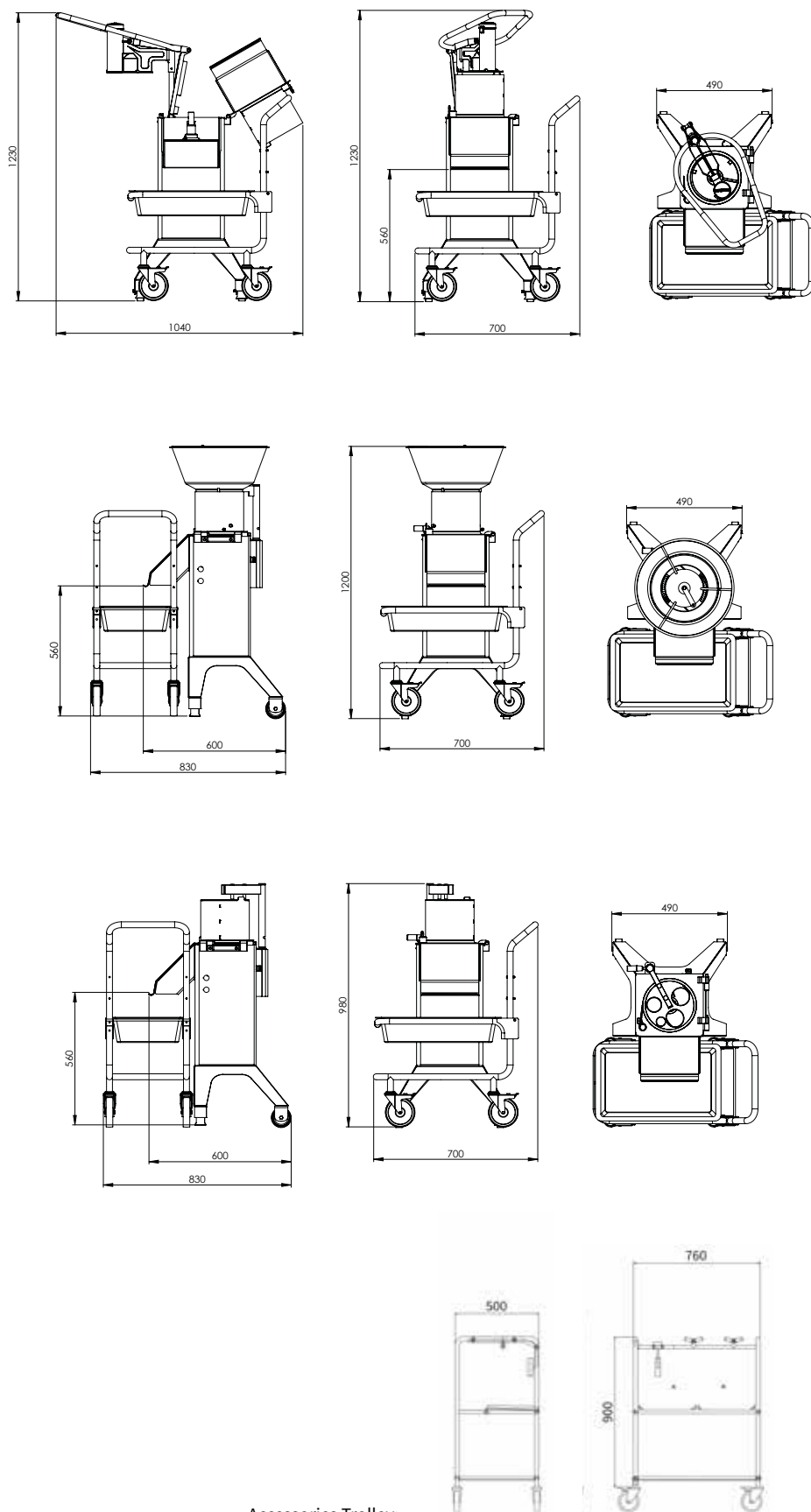
Accessories Trolley:
