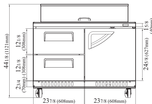
TST-48SD-18-D2R-FB-N FRONT VIEW
