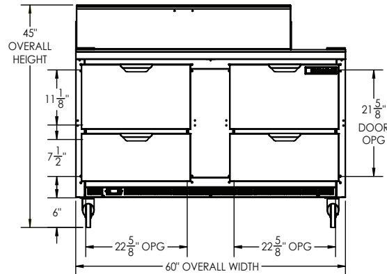
ELEVATION VIEW
