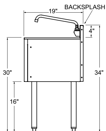
SIDE ELEVATION
