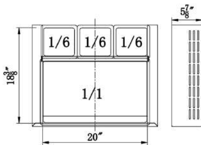
Upper drawer
