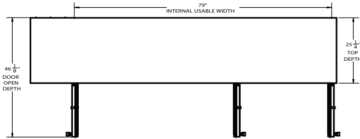
ELEVATION VIEW
