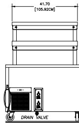
SFTS2-50-NUP WITH OPTIONAL TOP SHELF AND SNEEZE GLASS
