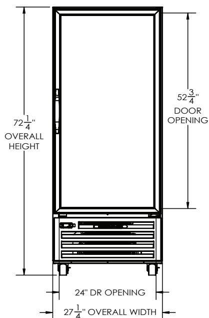
ELEVATION VIEW
