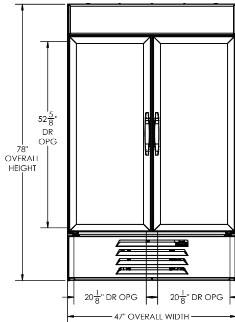
ELEVATION VIEW
