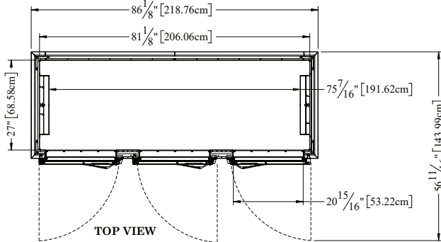
Shown on optional 6" casters
