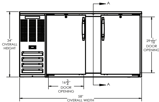
ELEVATION VIEW
