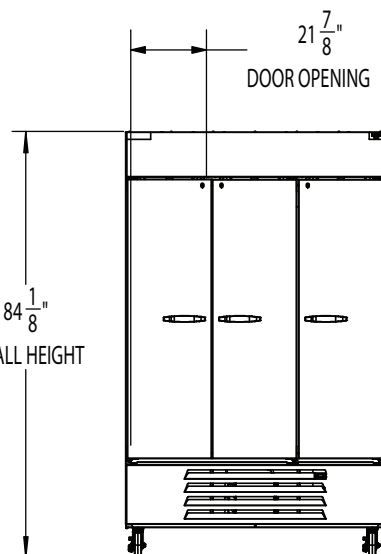
ELEVATION VIEW
