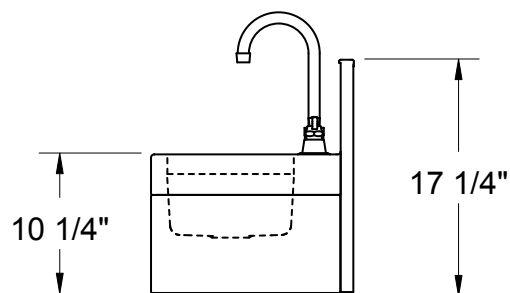
WHS-14 SIDE VIEW
