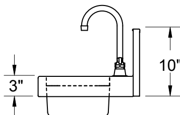
WH-14 SIDE VIEW
