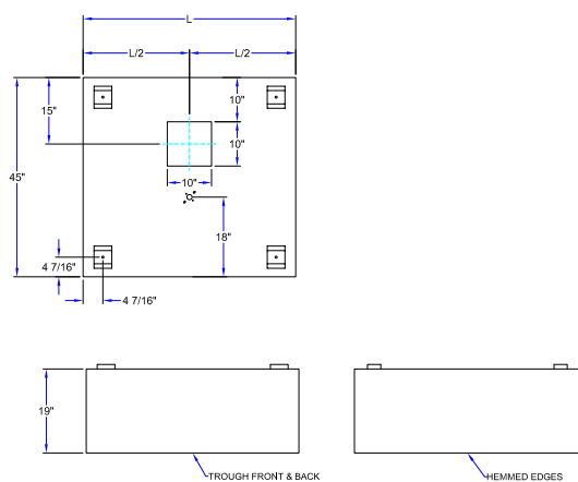
DRAWING 1 (INCLUDES 1 VAPOR PROOF LIGHT)
