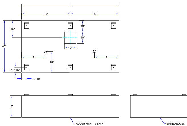
DRAWING 2 (INCLUDES 2 VAPOR PROOF LIGHTS)
