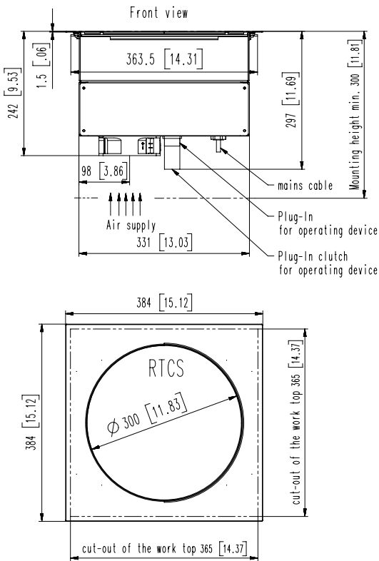
measurements in mm and [inch]
