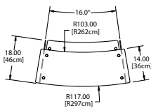
DCFSRIKS-2 Plan View
