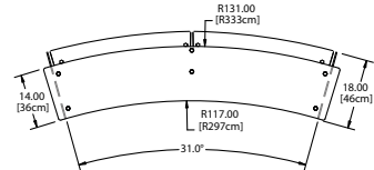
DCFSROKS-4 Plan View
