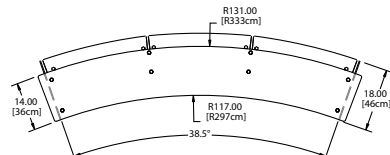
DCFSROKS-5 Plan View
