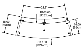
DCFSRIKS-3 Plan View
