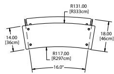
DCFSROKS-2 Plan View
