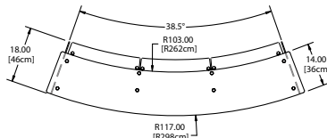
DCFSRIKS-5 Plan View
