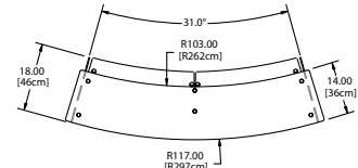
DCFSRIKS-4 Plan View
