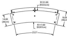
DCFSROKS-3 Plan View
