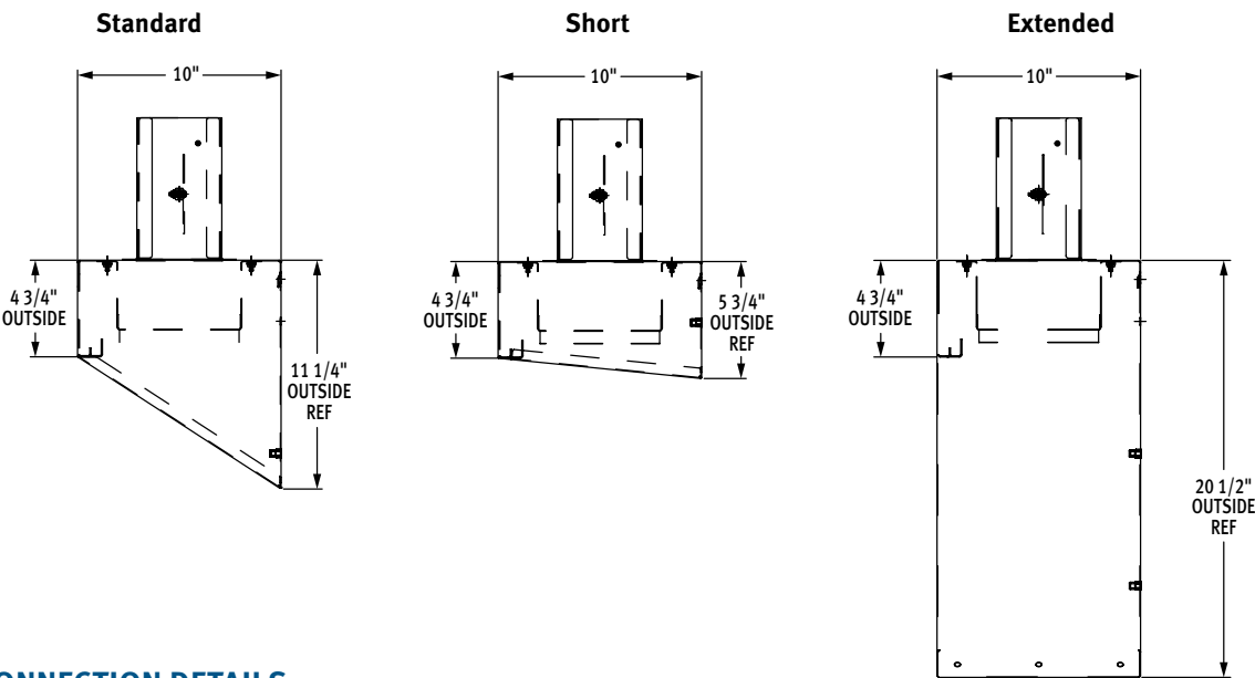
Tabling Connection: 64" inside tank (at table connection)
