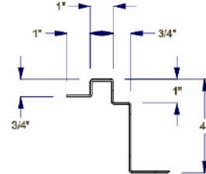
DETAIL B SCALE .2
