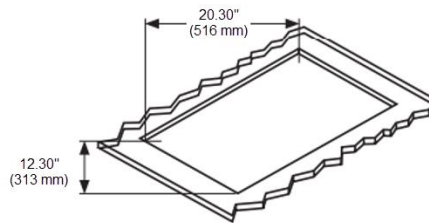
Countertop Cutout Dimensions
