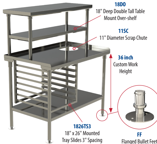
TB412-3048 14 Gauge Stainless Steel Top with 1.5" Backsplash and Open Base and U-Brace
