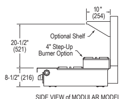
SIDE VIEW of MODULAR MODEL
