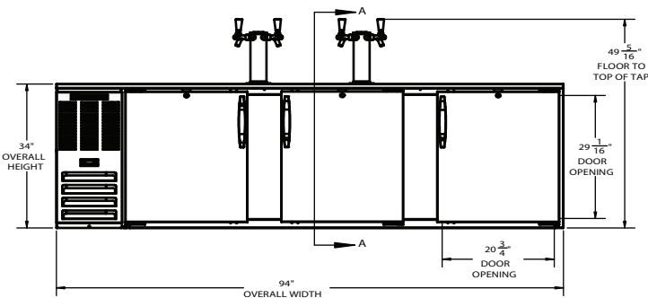
ELEVATION VIEW
