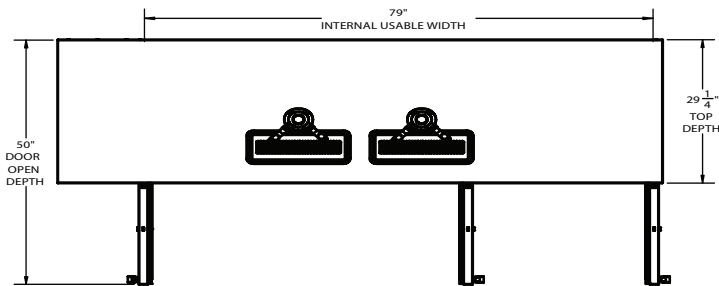
ELEVATION VIEW
