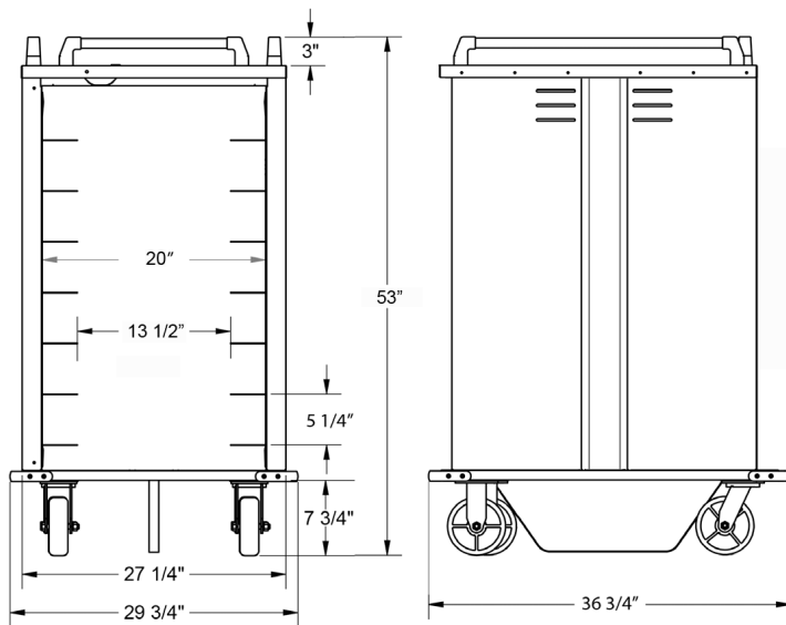
Model ST1D2T14
