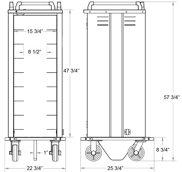
Model ST1D1T8
