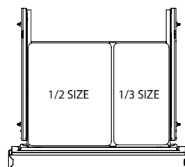
SINGLE DRAWER PAN LAYOUT
