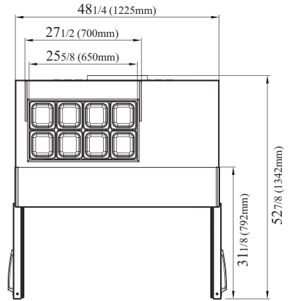
PST-48-08S-N TOP VIEW
