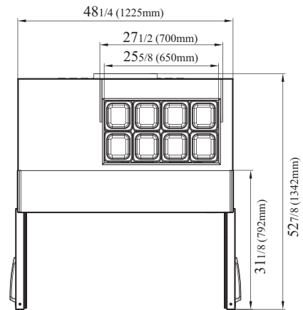
PST-48-08S-N-LW TOP VIEW
