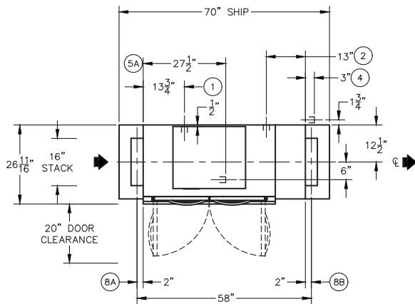
Plan View: Left to Right Model L-R
