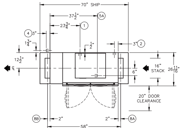
Plan View: Right to Left Model R-L
