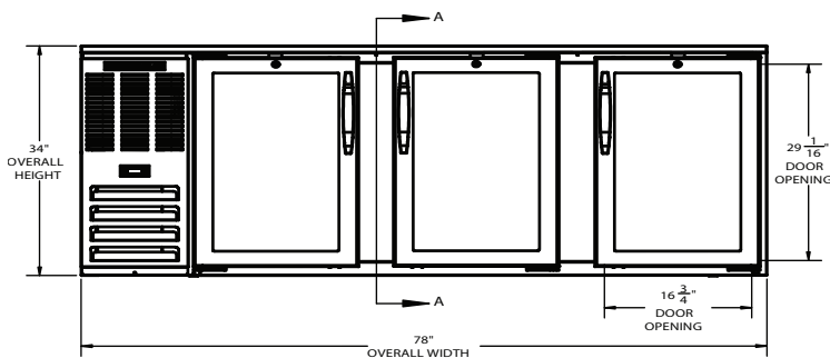
ELEVATION VIEW
