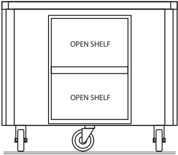
Elevation View SC-TRIOS
