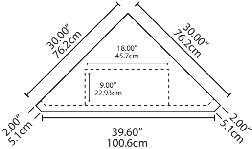
Plan View SC-TRIOS
