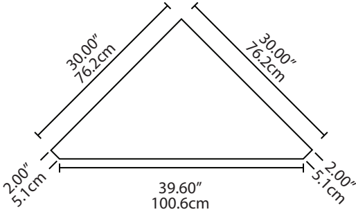
Plan View SC-TRI
