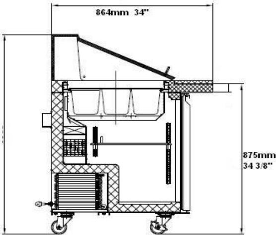
Section View
